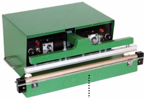
Automatic Sealer 18", 24" Seal Width Pressure Time 1-8 sec. Cycle Frequency 1-8 sec. Heat Seal Time 0.2 – 0.3 sec. Foot Pedal or Automatic Action
